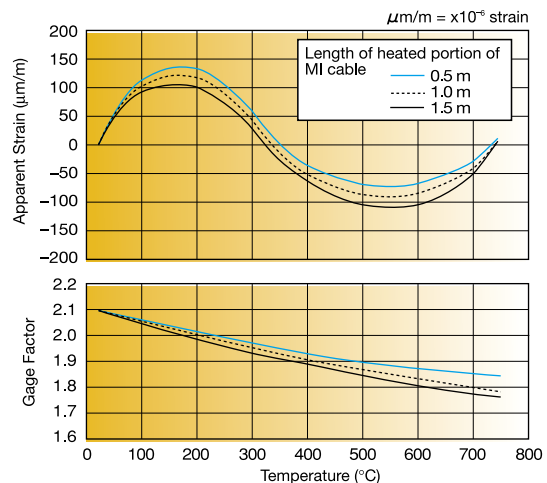
Estimated Thermally-induced Apparent Strain and Gage Factor Change
