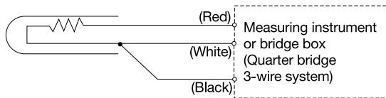
Structure & Circuit
